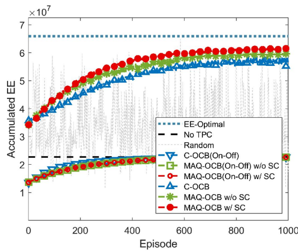
Figure 4. Energy efficiency vs. episode when |\mathcal{U}| = 60 , |\mathcal{M}| = 3 , and |\mathcal{N}| = 6 .
